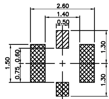
RECOMMENDED PCB LAYOUT (TOLERANCE:±0.05)
