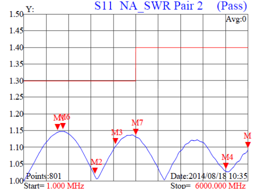
S11 NA_SWR Pair 2 (Pass)
